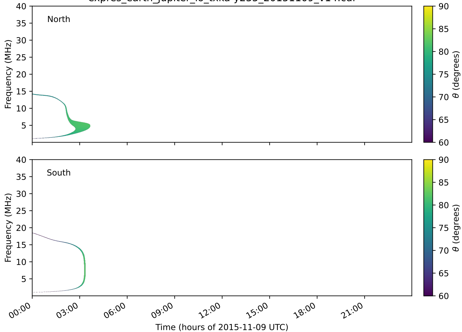
expres_earth_jupiter_io_txka-y235_20151109_v14.cdf
