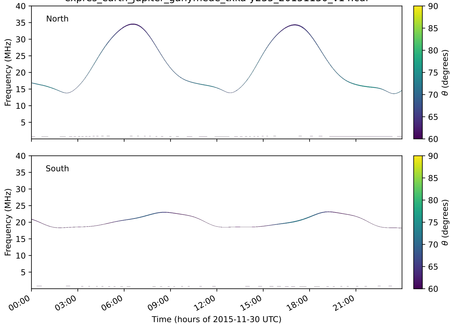
expres_earth_jupiter_ganymede_txka-y235_20151130_v14.cdf
