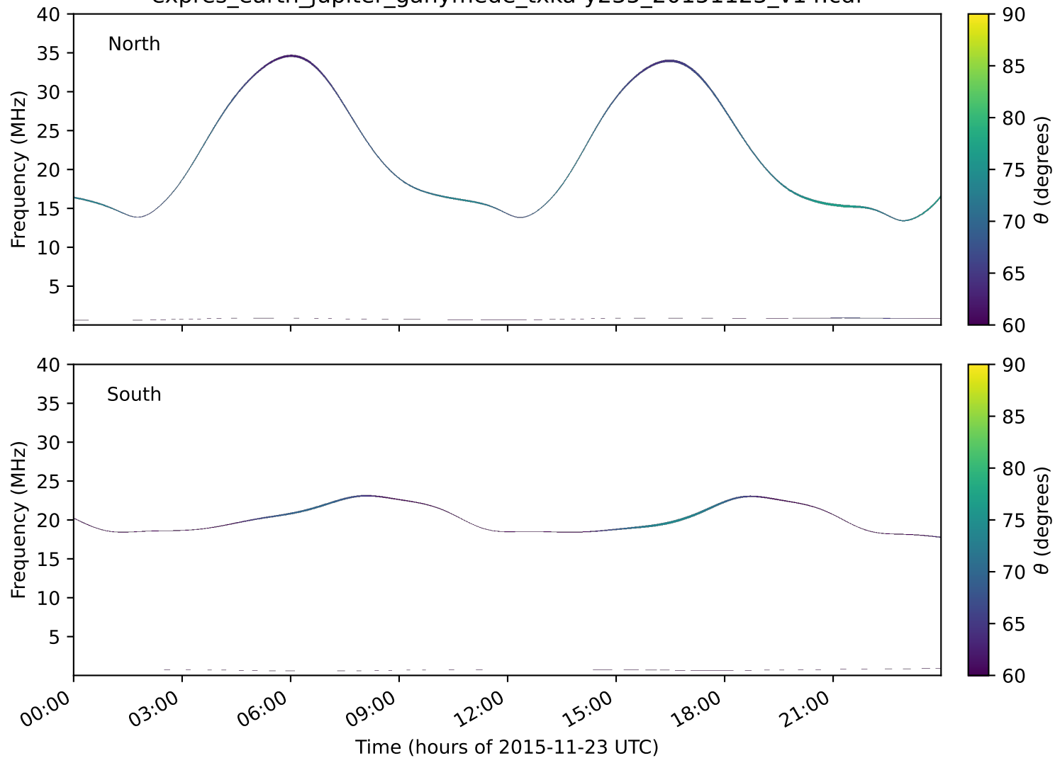
expres_earth_jupiter_ganymede_txka-y235_20151123_v14.cdf
