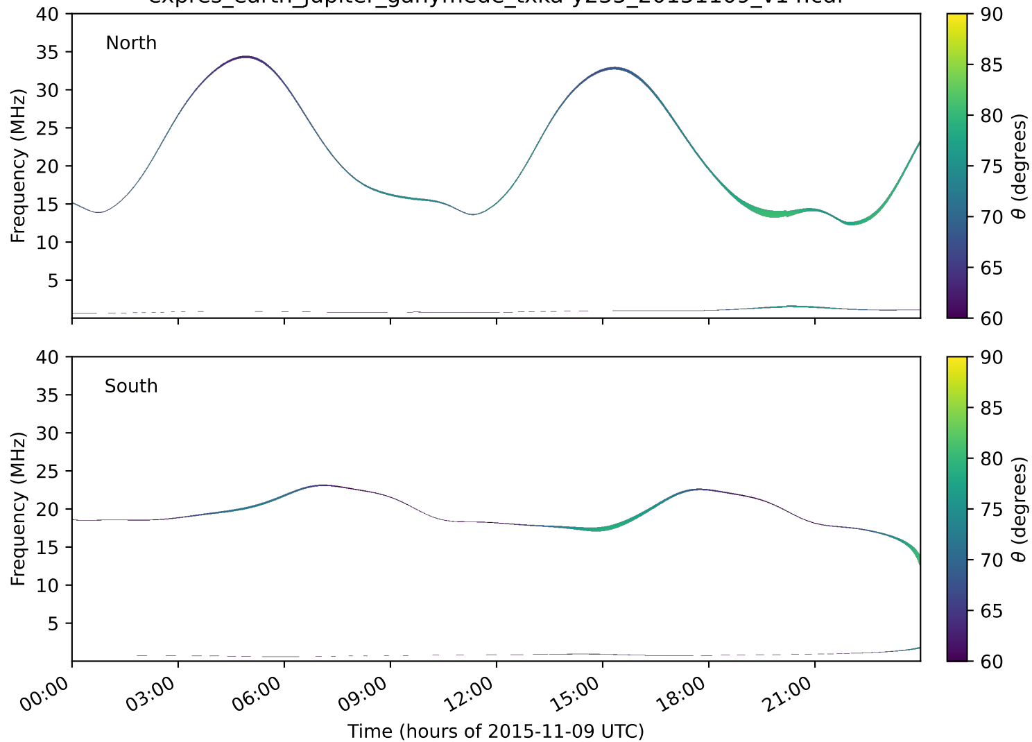
expres_earth_jupiter_ganymede_txka-y235_20151109_v14.cdf
