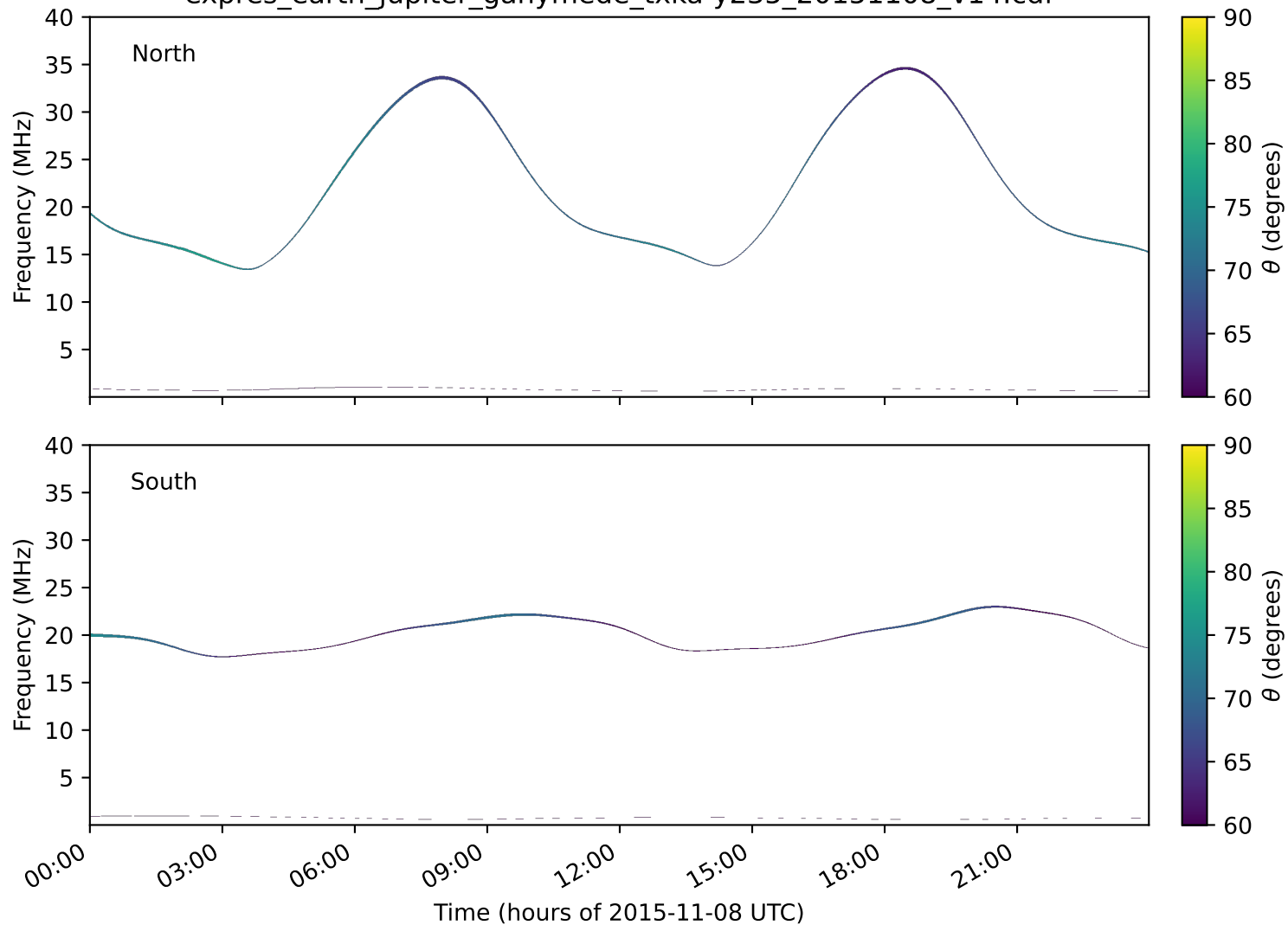
expres_earth_jupiter_ganymede_txka-y235_20151108_v14.cdf
