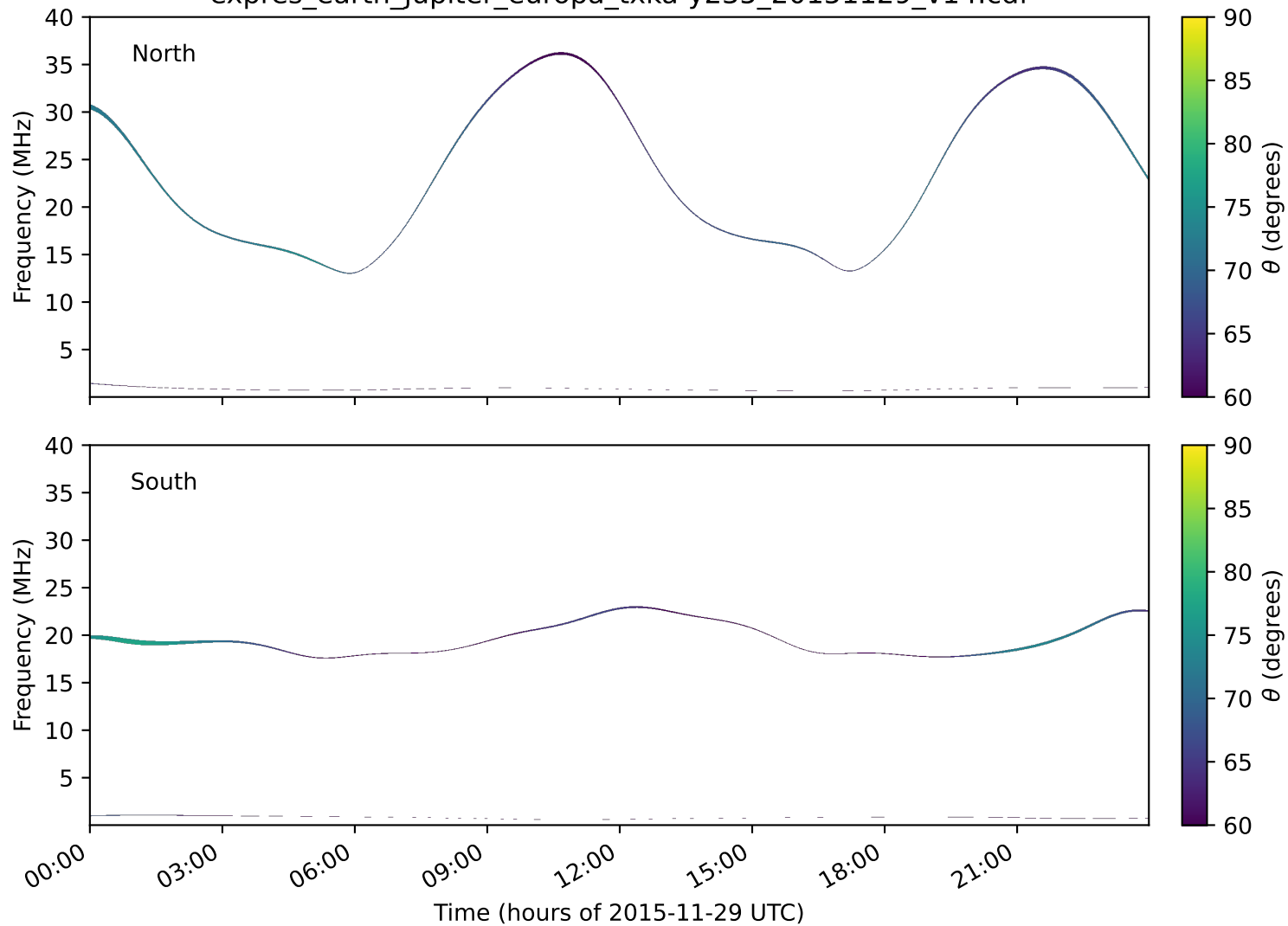
expres_earth_jupiter_europa_txka-y235_20151129_v14.cdf
