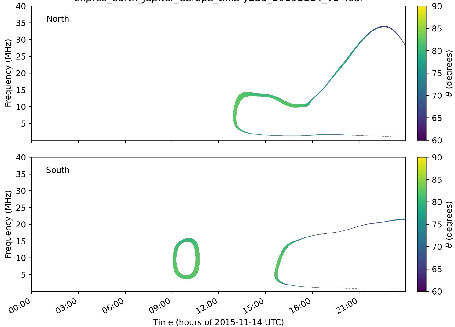
expres_earth_jupiter_europa_txka-y235_20151114_v14.cdf
