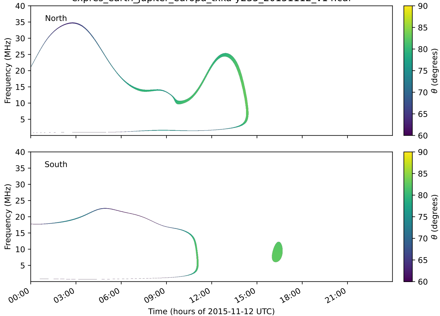
expres_earth_jupiter_europa_txka-y235_20151112_v14.cdf
