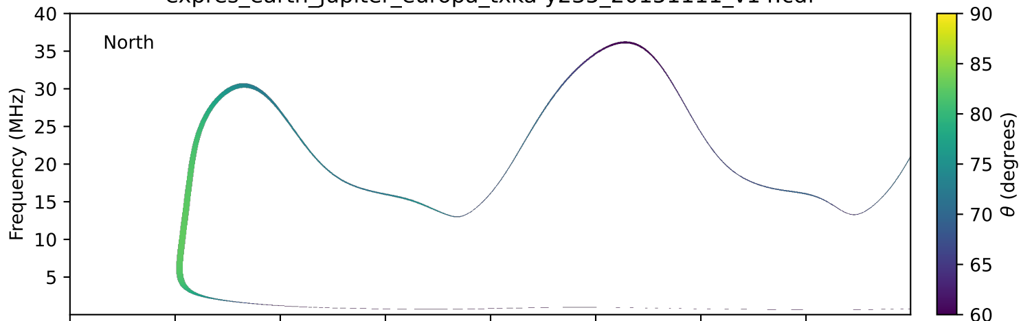
expres_earth_jupiter_europa_txka-y235_20151111_v14.cdf
