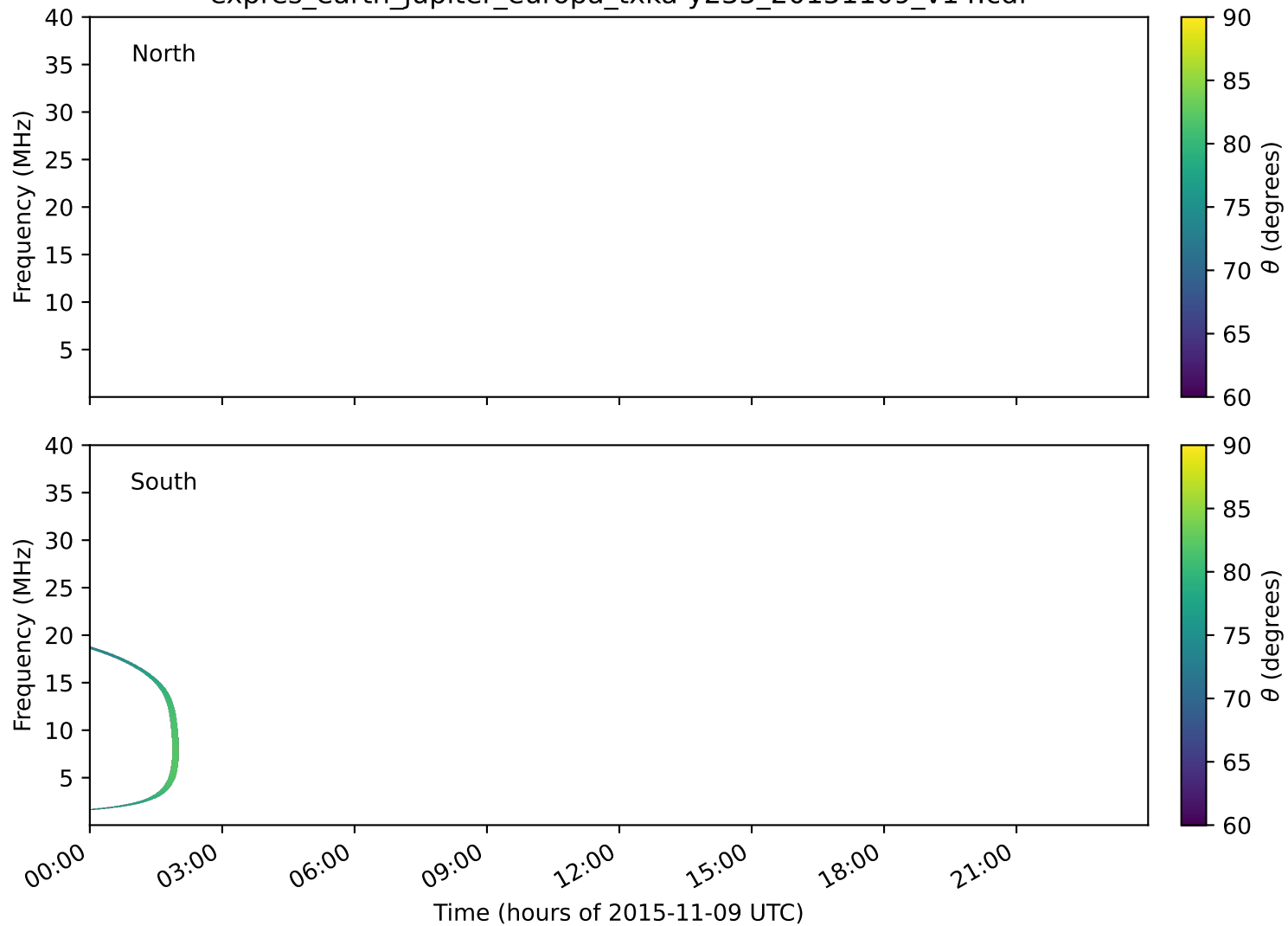
expres_earth_jupiter_europa_txka-y235_20151109_v14.cdf
