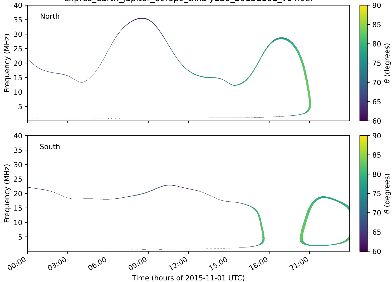
expres_earth_jupiter_europa_txka-y235_20151101_v14.cdf
