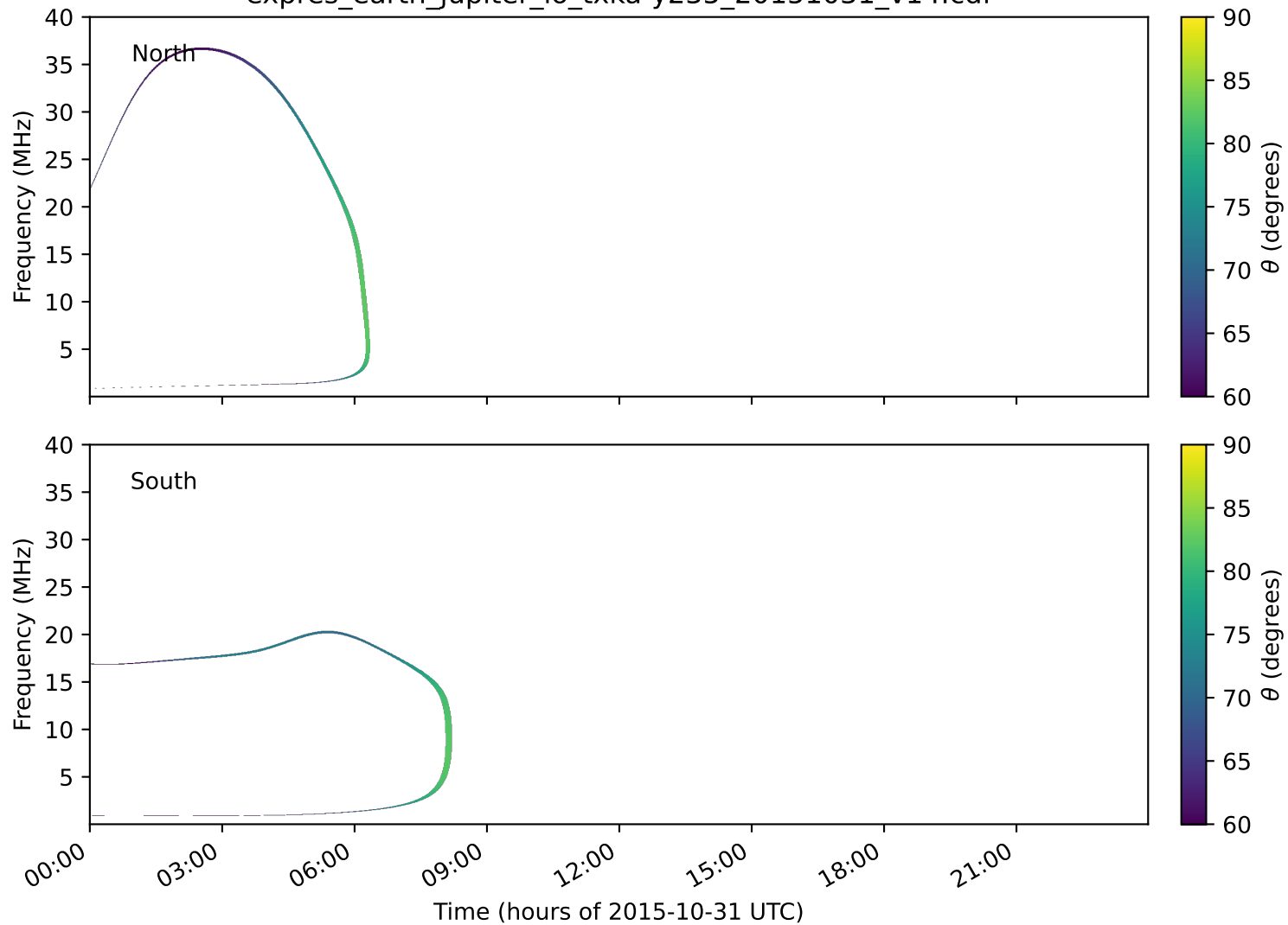
expres_earth_jupiter_io_txka-y235_20151031_v14.cdf
