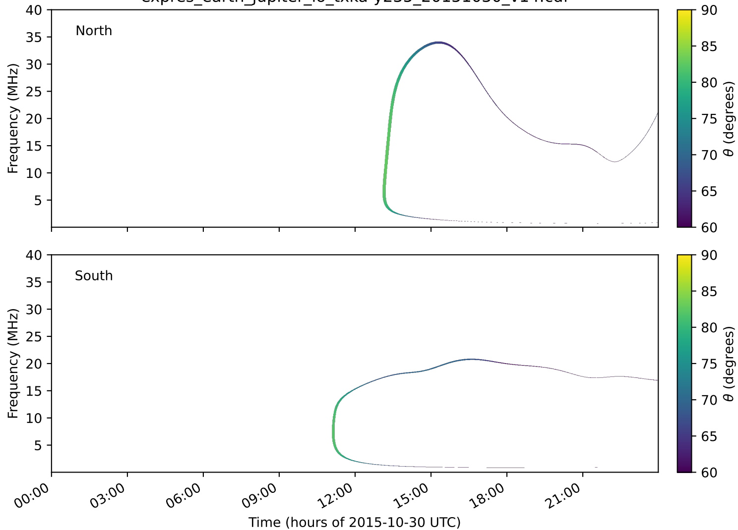
expres_earth_jupiter_io_txka-y235_20151030_v14.cdf
