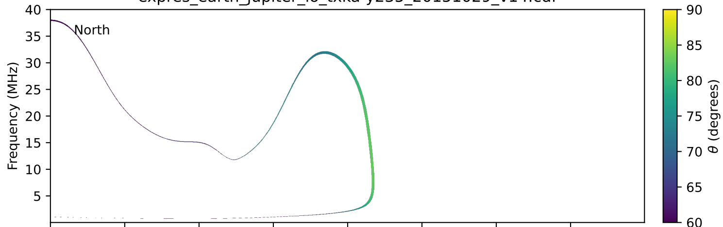
expres_earth_jupiter_io_txka-y235_20151029_v14.cdf
