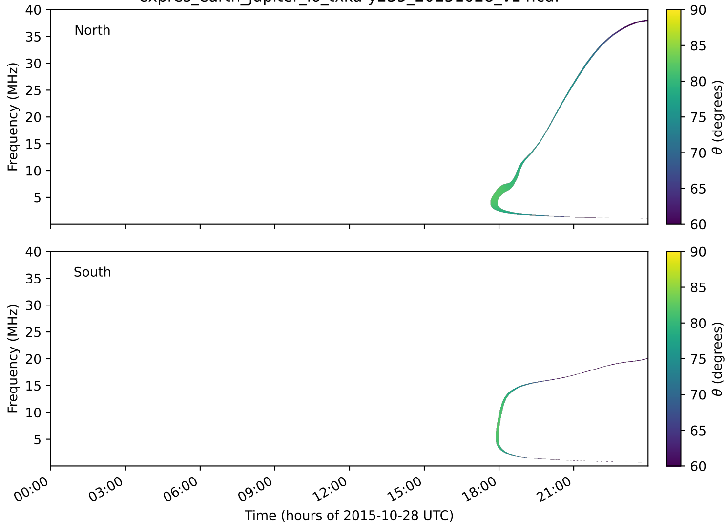
expres_earth_jupiter_io_txka-y235_20151028_v14.cdf
