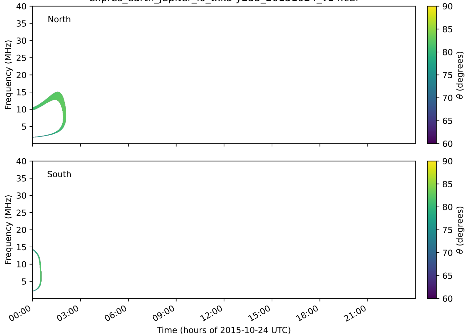
expres_earth_jupiter_io_txka-y235_20151024_v14.cdf
