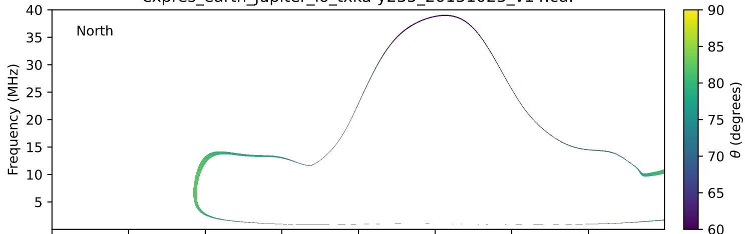
expres_earth_jupiter_io_txka-y235_20151023_v14.cdf
