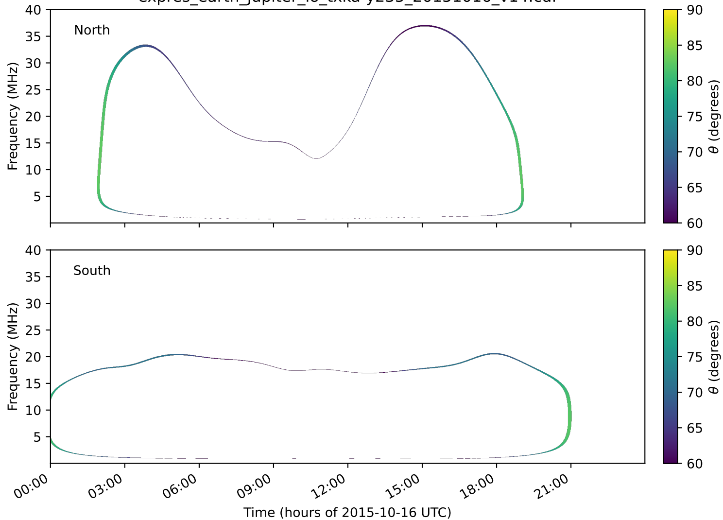
expres_earth_jupiter_io_txka-y235_20151016_v14.cdf
