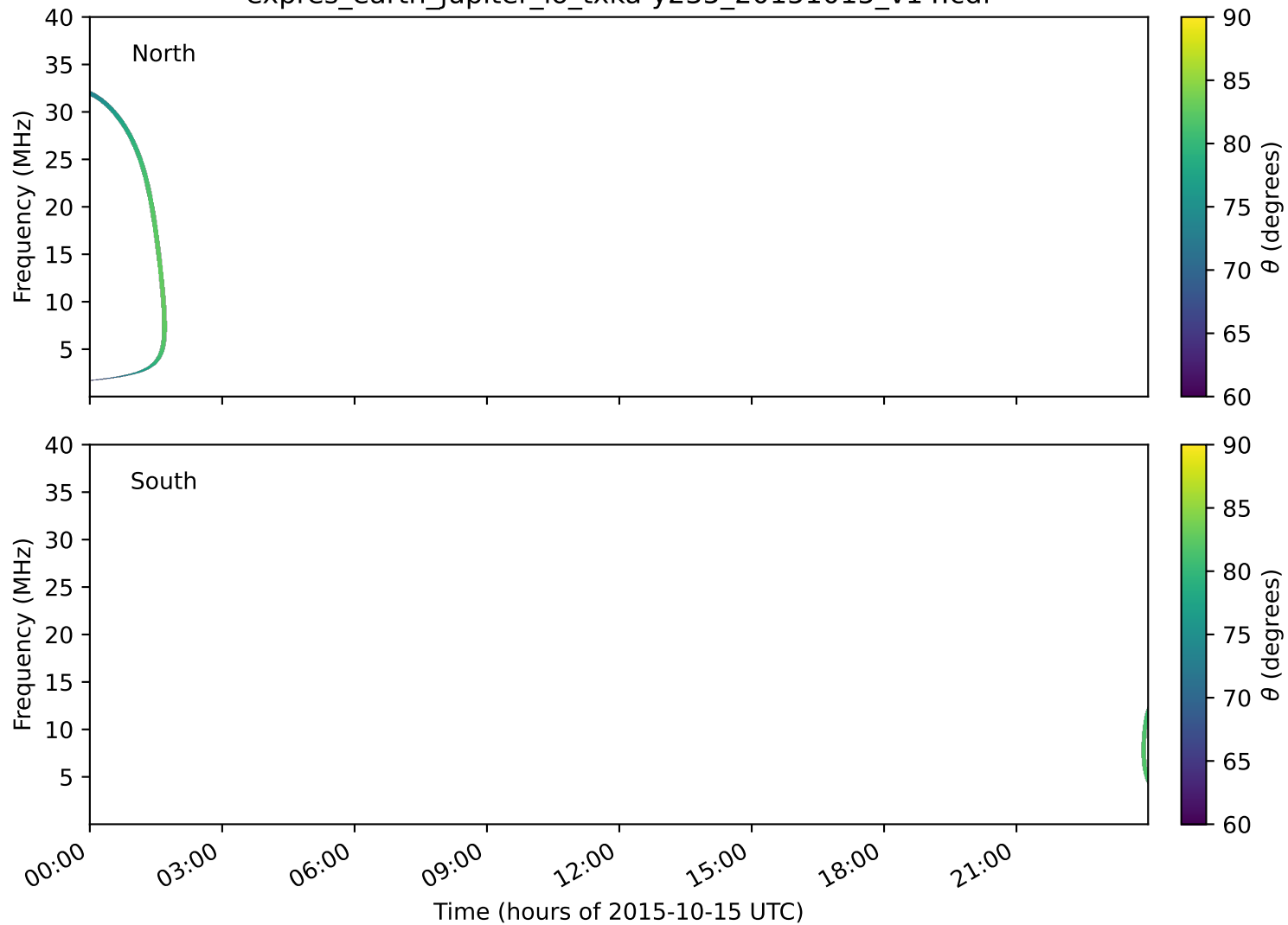
expres_earth_jupiter_io_txka-y235_20151015_v14.cdf
