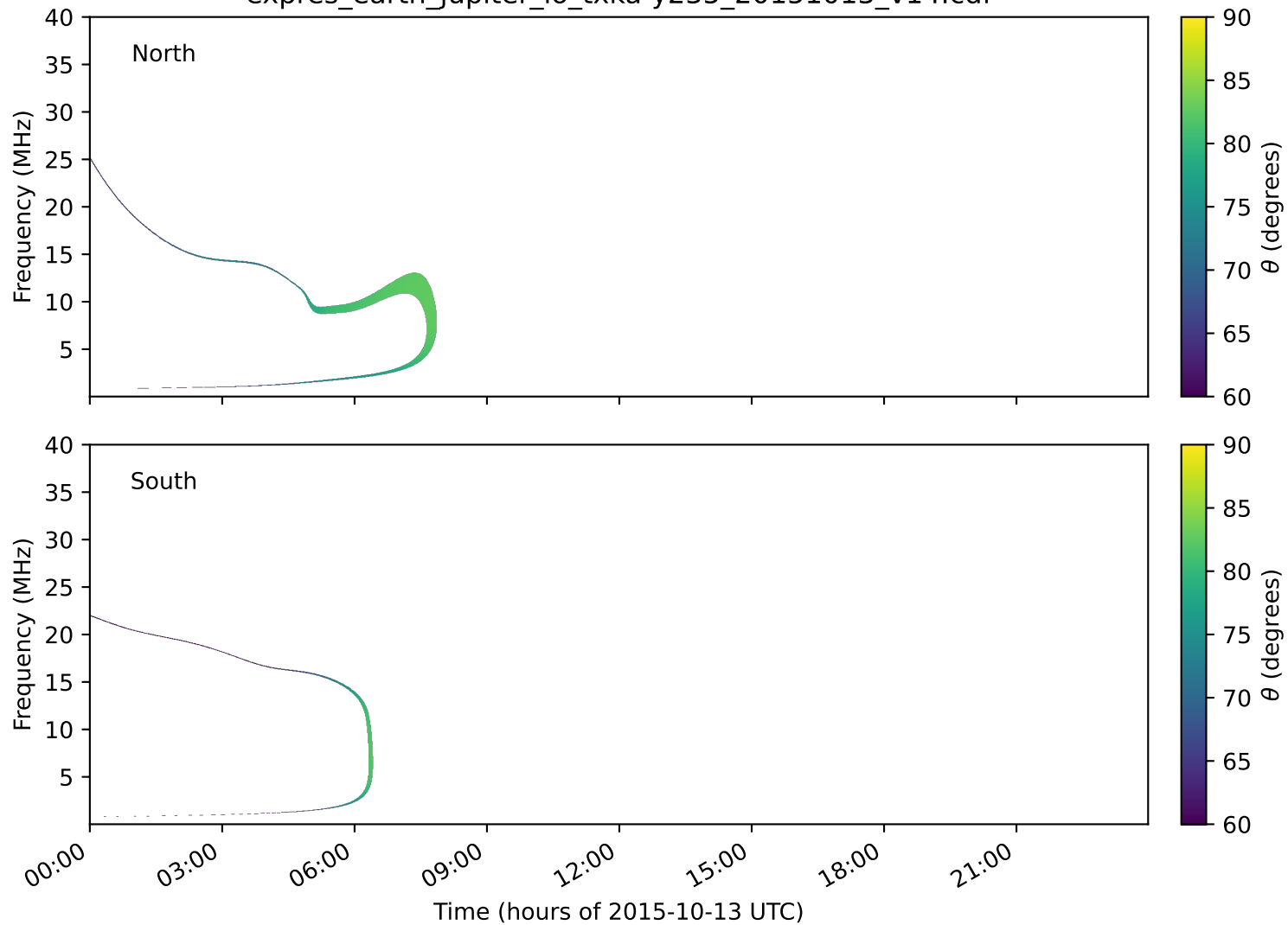
expres_earth_jupiter_io_txka-y235_20151013_v14.cdf
