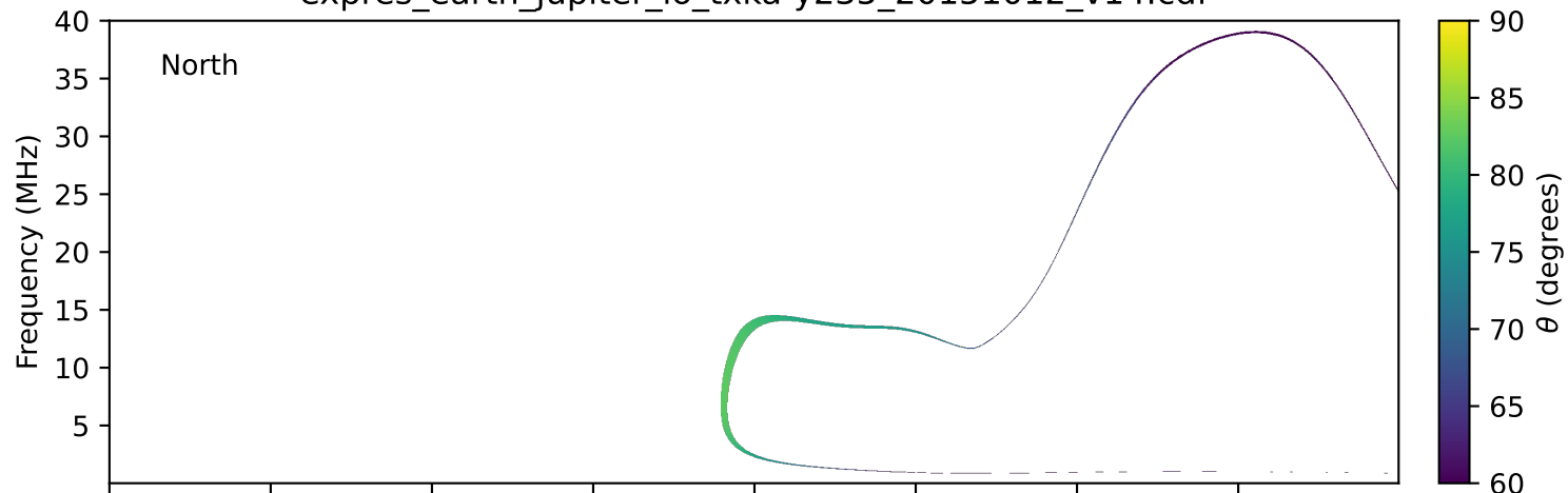
expres_earth_jupiter_io_txka-y235_20151012_v14.cdf
