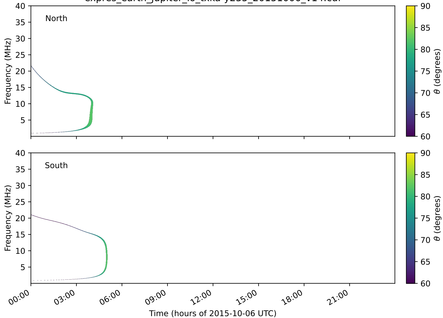
expres_earth_jupiter_io_txka-y235_20151006_v14.cdf
