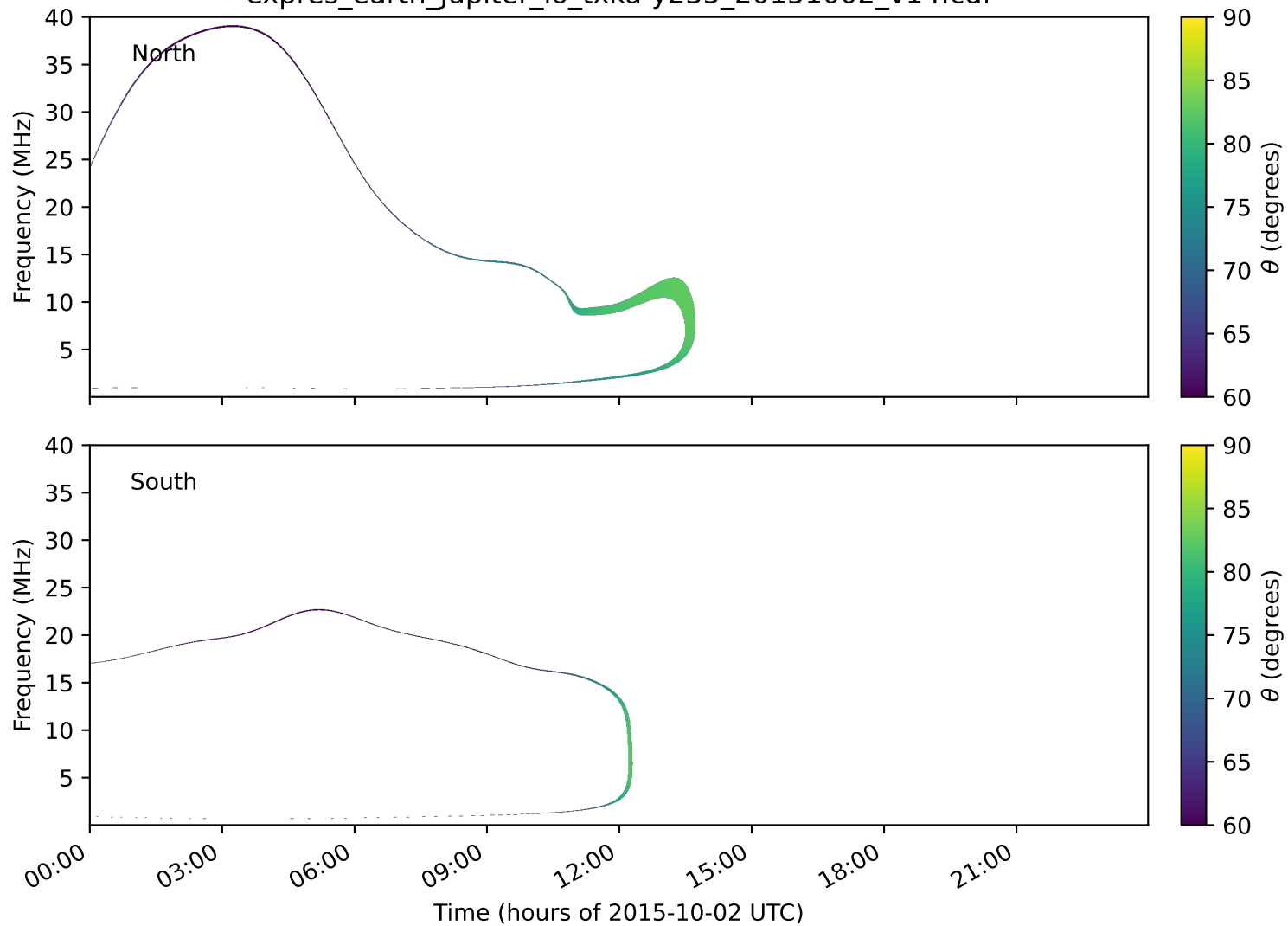
expres_earth_jupiter_io_txka-y235_20151002_v14.cdf
