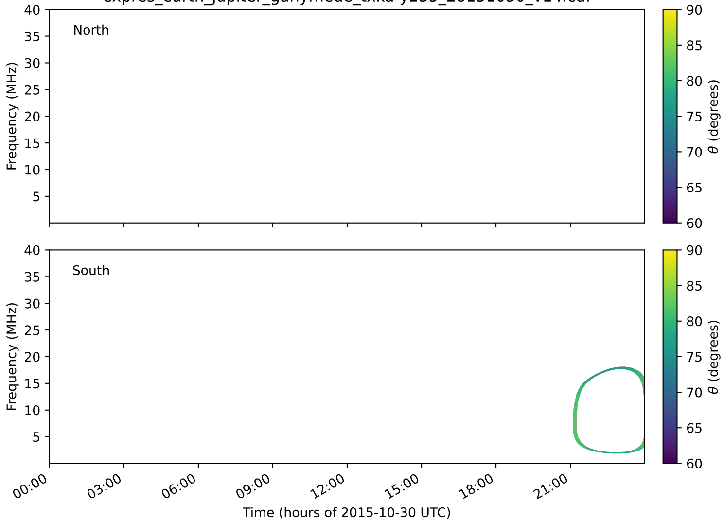
expres_earth_jupiter_ganymede_txka-y235_20151030_v14.cdf
