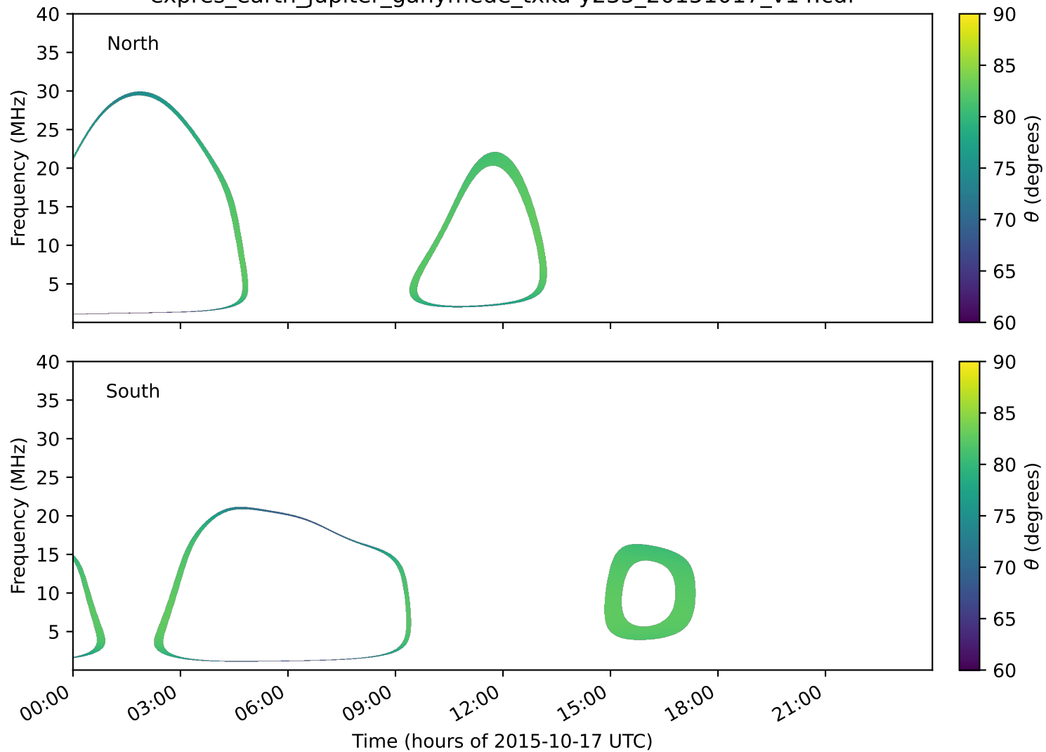
expres_earth_jupiter_ganymede_txka-y235_20151017_v14.cdf
