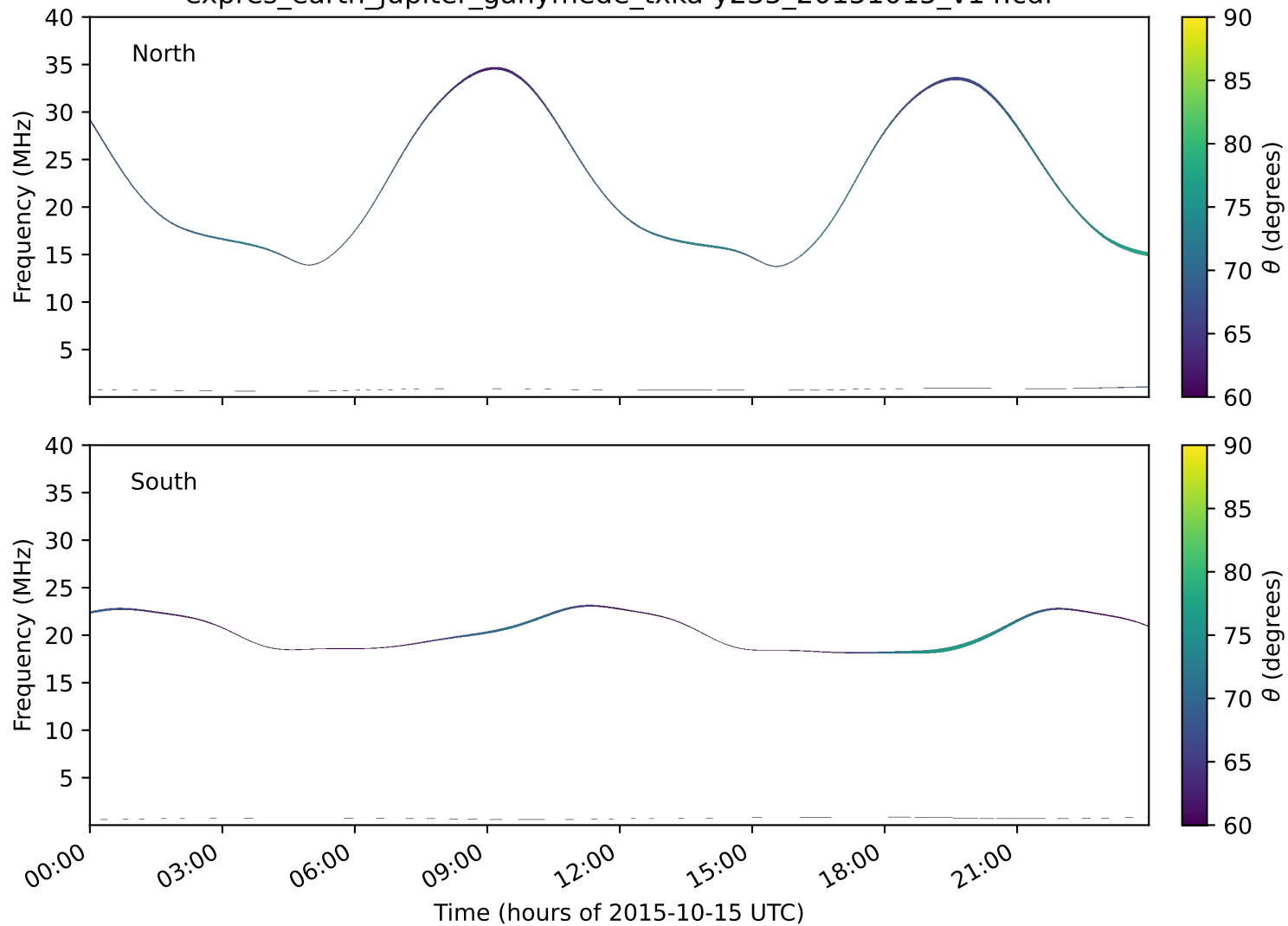
expres_earth_jupiter_ganymede_txka-y235_20151015_v14.cdf
