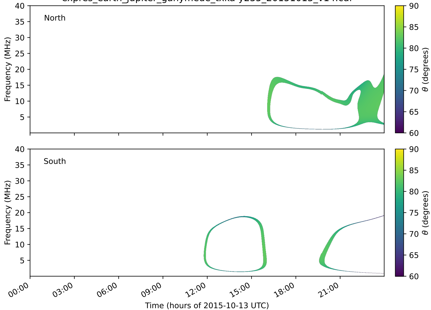
expres_earth_jupiter_ganymede_txka-y235_20151013_v14.cdf
