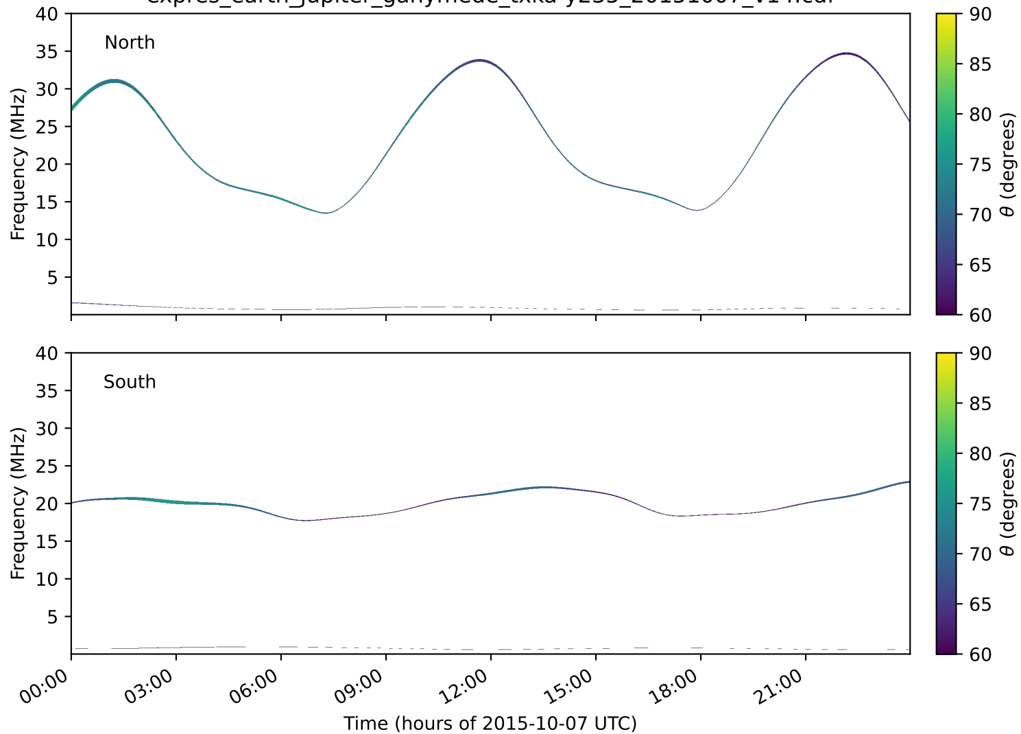
expres_earth_jupiter_ganymede_txka-y235_20151007_v14.cdf
