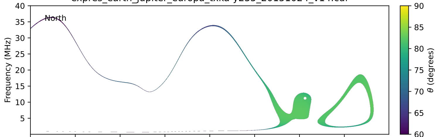
expres_earth_jupiter_europa_txka-y235_20151024_v14.cdf
