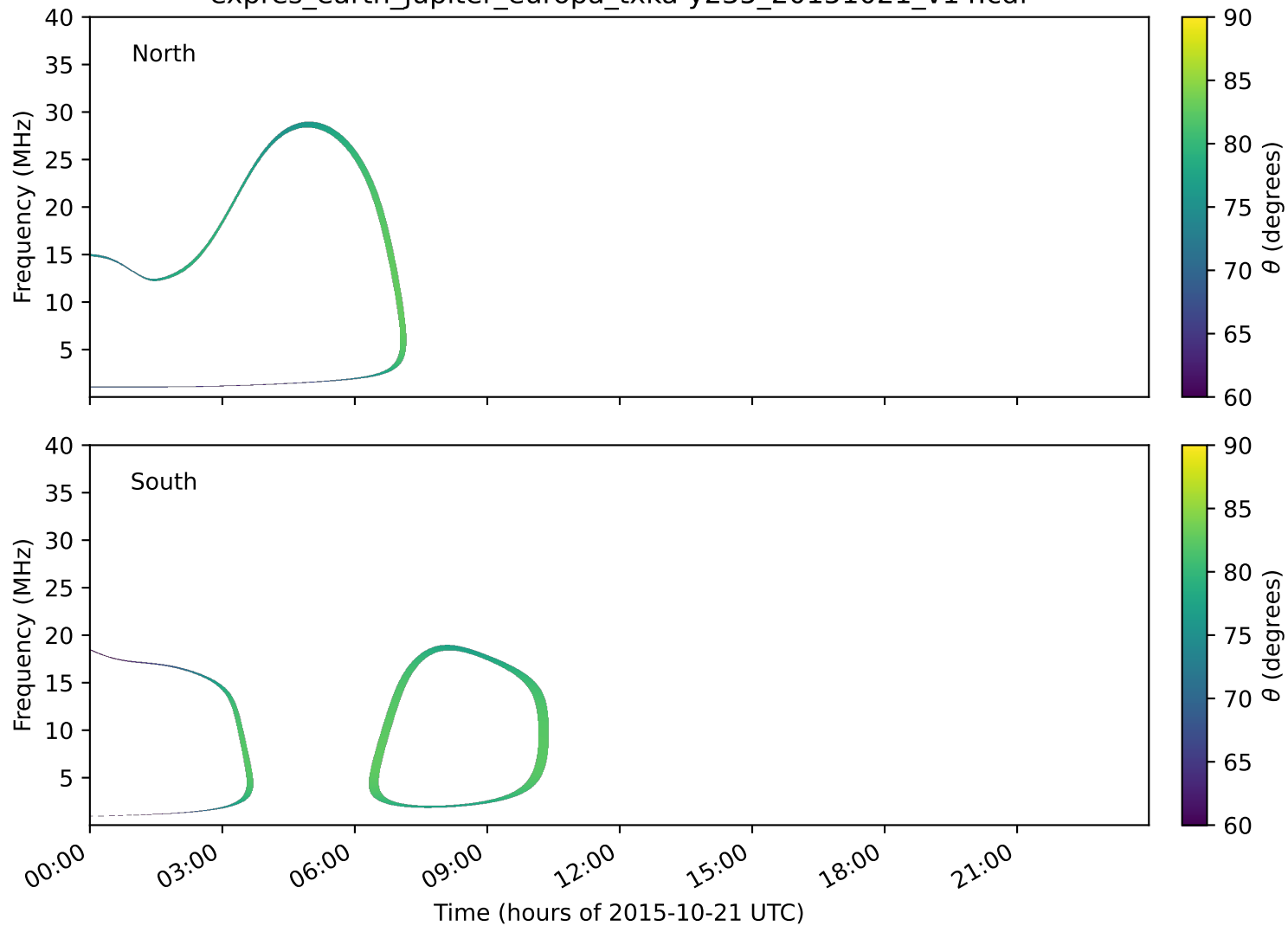
expres_earth_jupiter_europa_txka-y235_20151021_v14.cdf
