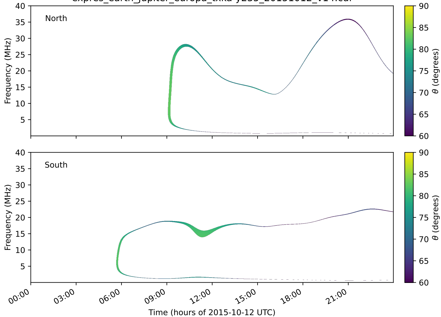
expres_earth_jupiter_europa_txka-y235_20151012_v14.cdf
