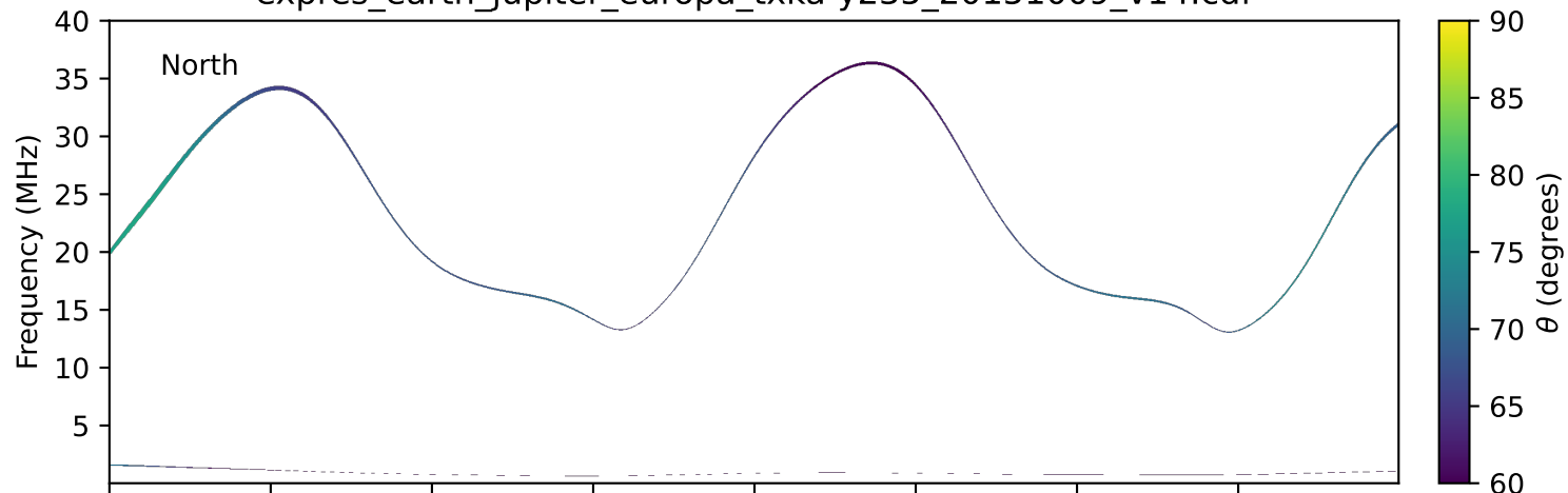
expres_earth_jupiter_europa_txka-y235_20151009_v14.cdf
