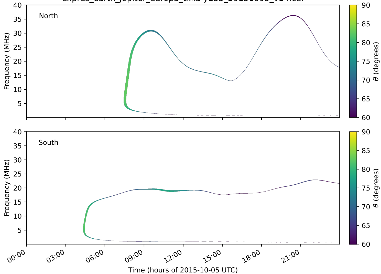
expres_earth_jupiter_europa_txka-y235_20151005_v14.cdf
