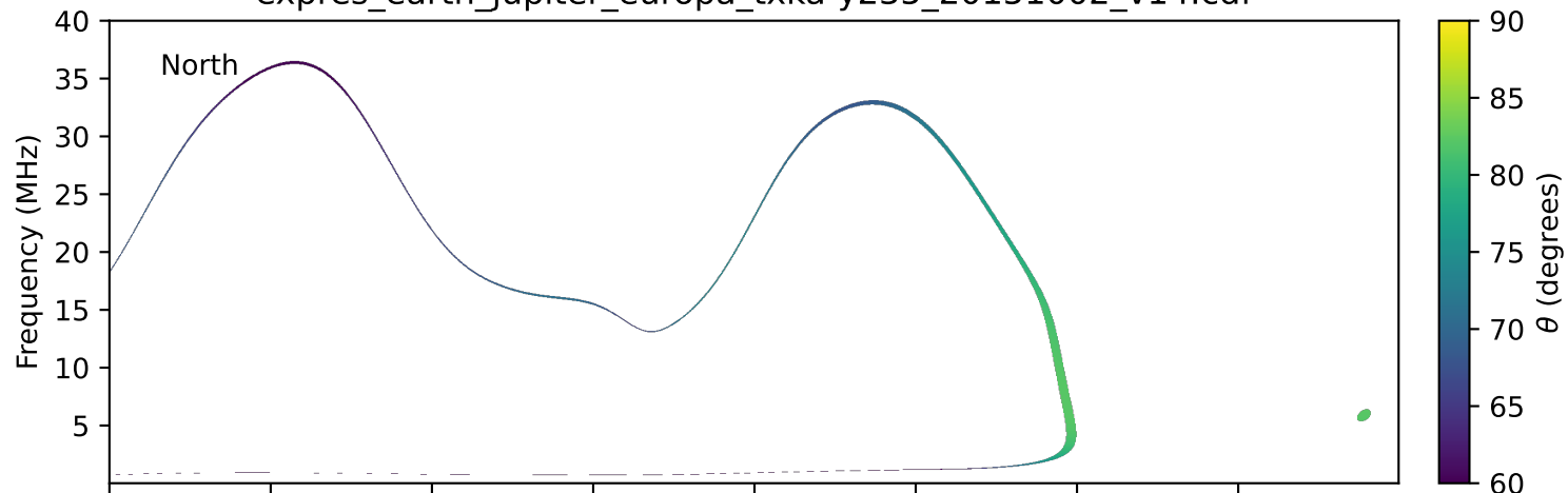
expres_earth_jupiter_europa_txka-y235_20151002_v14.cdf
