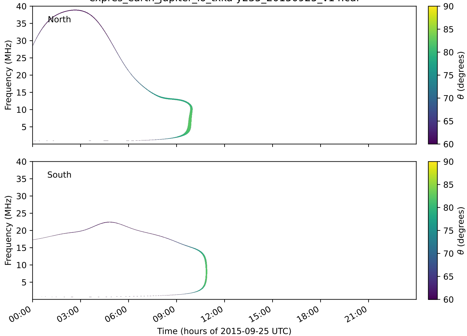
expres_earth_jupiter_io_txka-y235_20150925_v14.cdf
