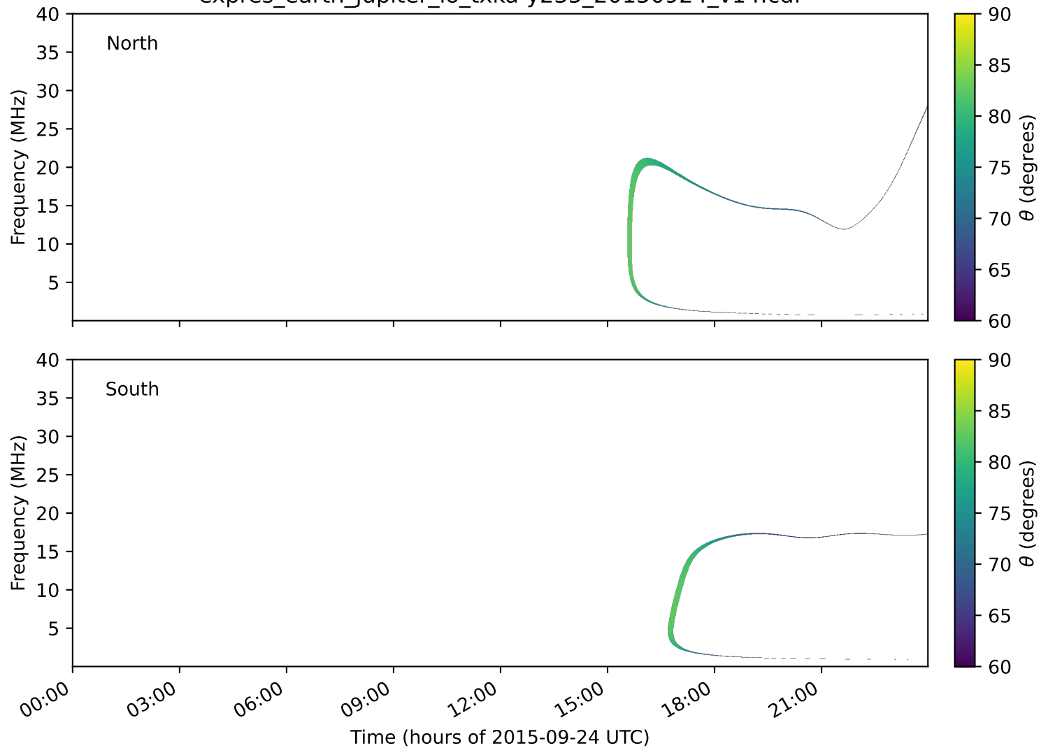
expres_earth_jupiter_io_txka-y235_20150924_v14.cdf
