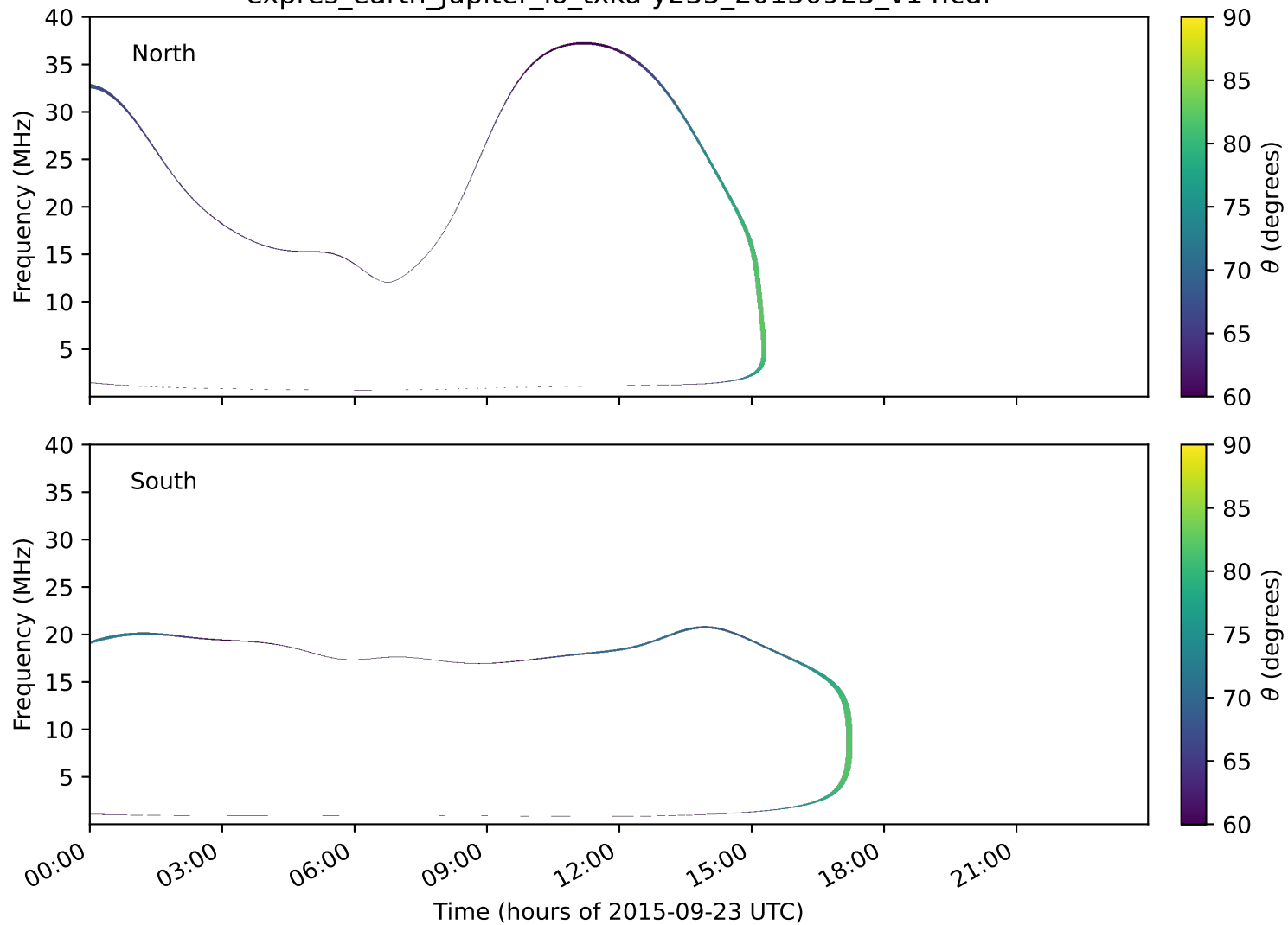
expres_earth_jupiter_io_txka-y235_20150923_v14.cdf
