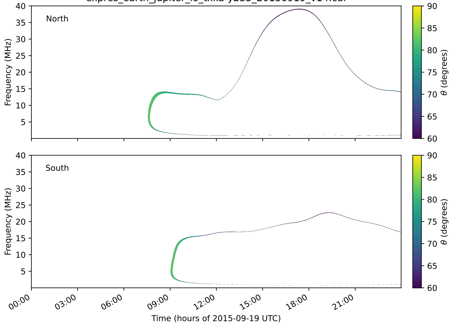
expres_earth_jupiter_io_txka-y235_20150919_v14.cdf
