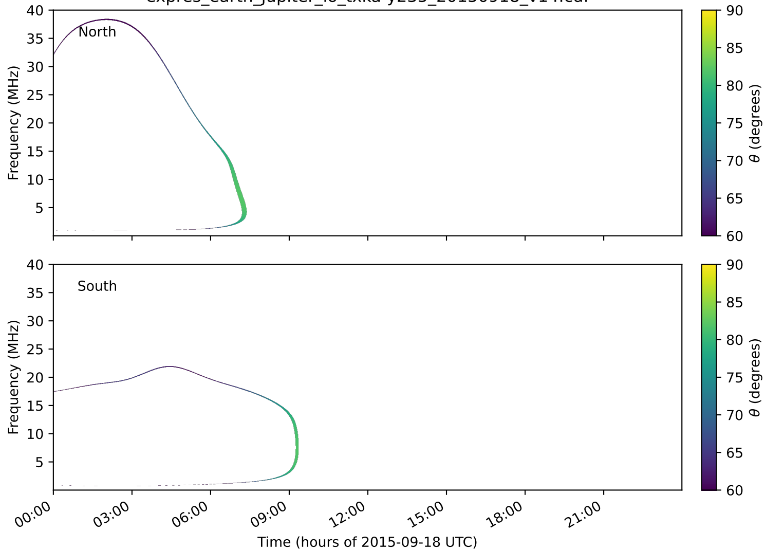
expres_earth_jupiter_io_txka-y235_20150918_v14.cdf
