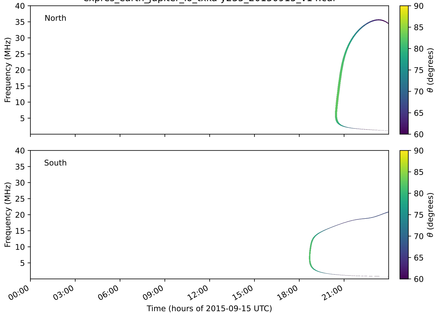
expres_earth_jupiter_io_txka-y235_20150915_v14.cdf
