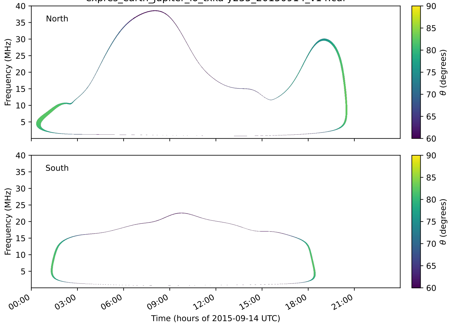
expres_earth_jupiter_io_txka-y235_20150914_v14.cdf
