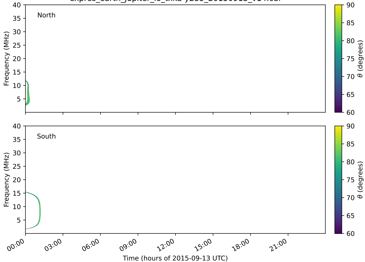
expres_earth_jupiter_io_txka-y235_20150913_v14.cdf
