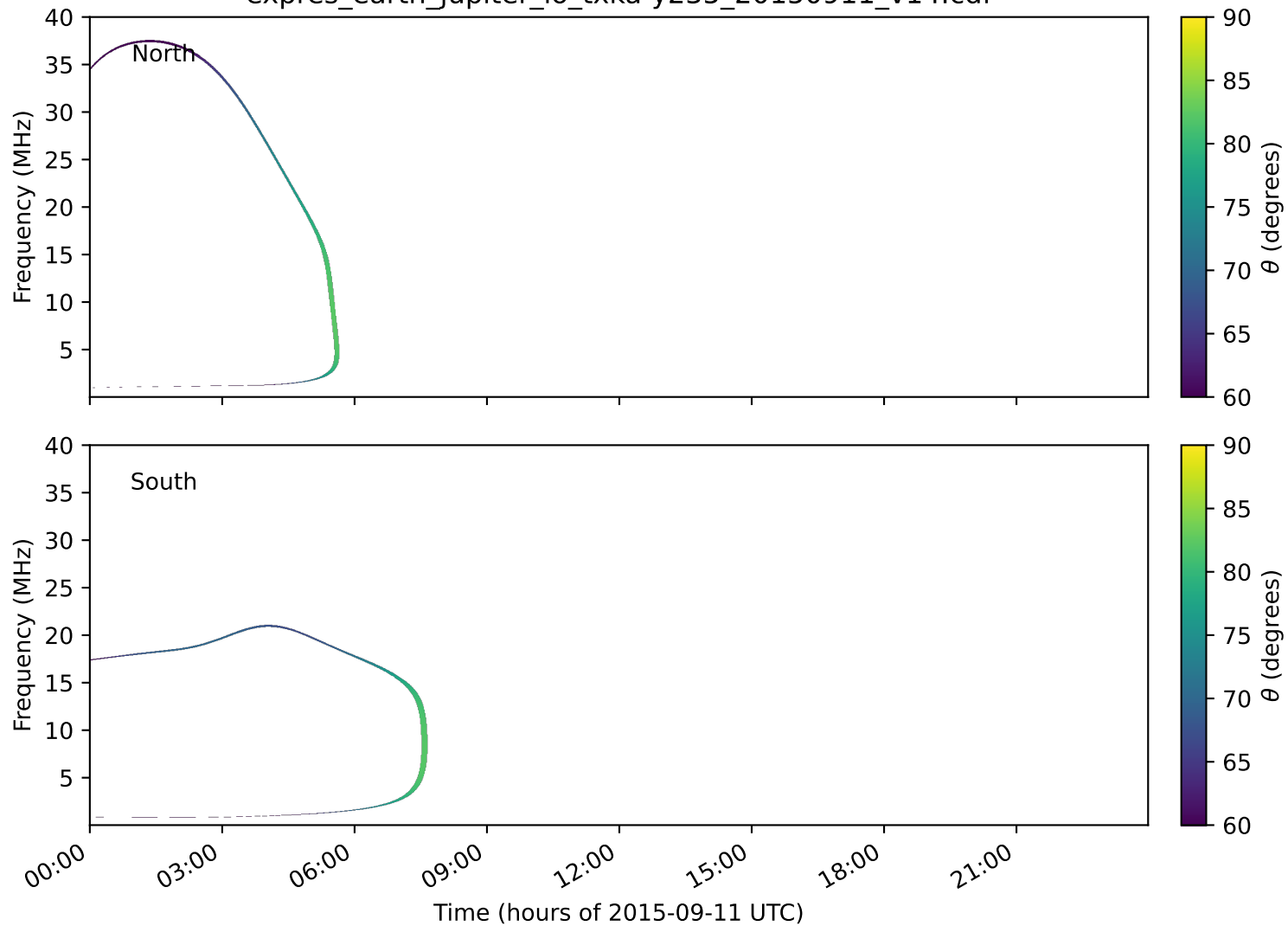
expres_earth_jupiter_io_txka-y235_20150911_v14.cdf
