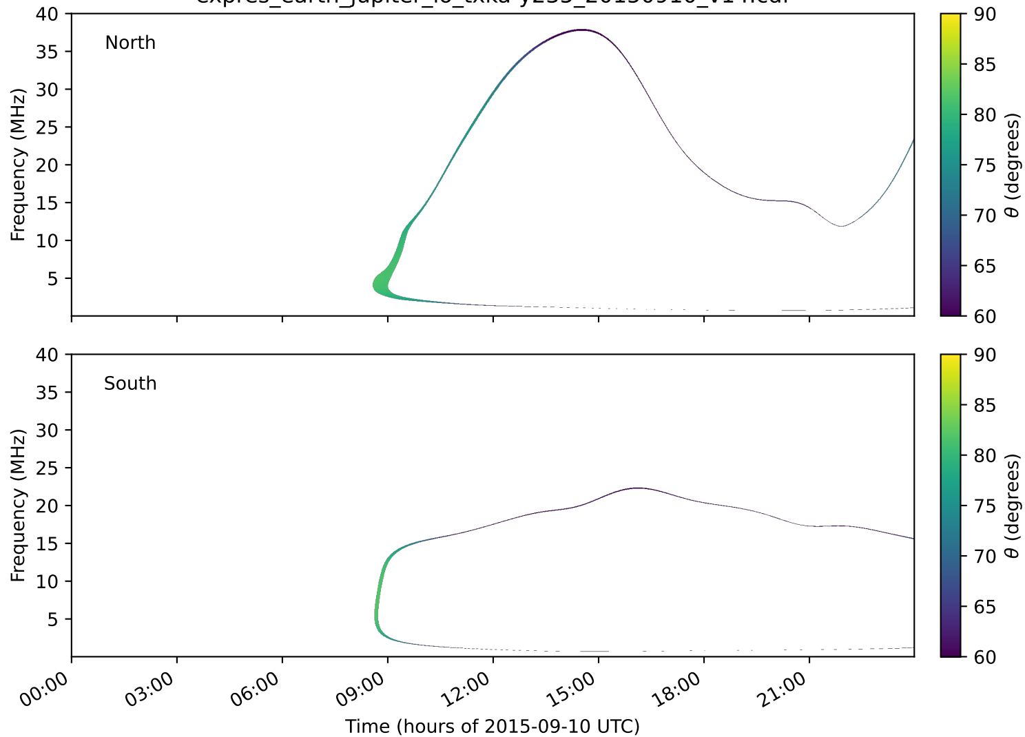
expres_earth_jupiter_io_txka-y235_20150910_v14.cdf
