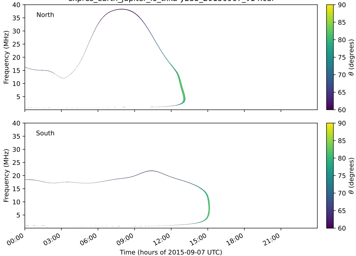
expres_earth_jupiter_io_txka-y235_20150907_v14.cdf
