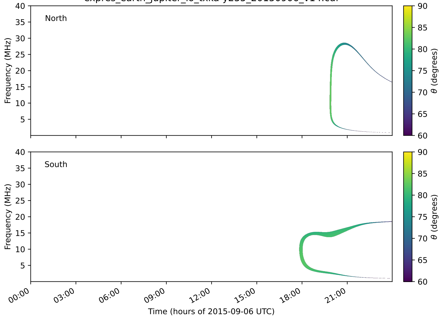
expres_earth_jupiter_io_txka-y235_20150906_v14.cdf
