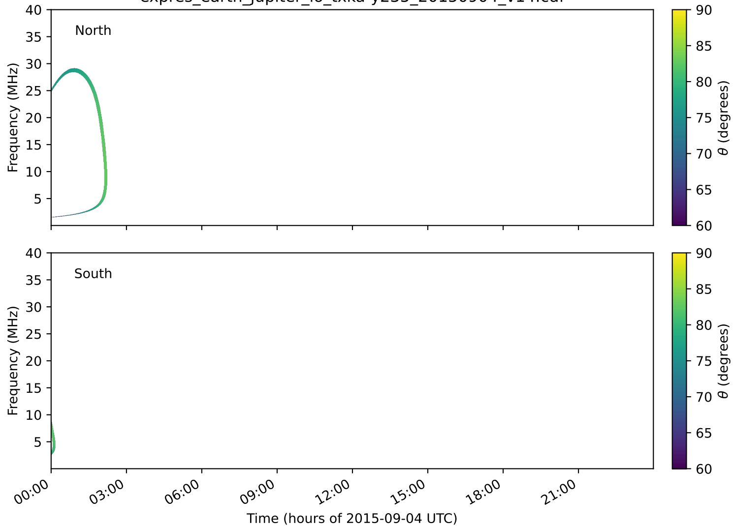
expres_earth_jupiter_io_txka-y235_20150904_v14.cdf
