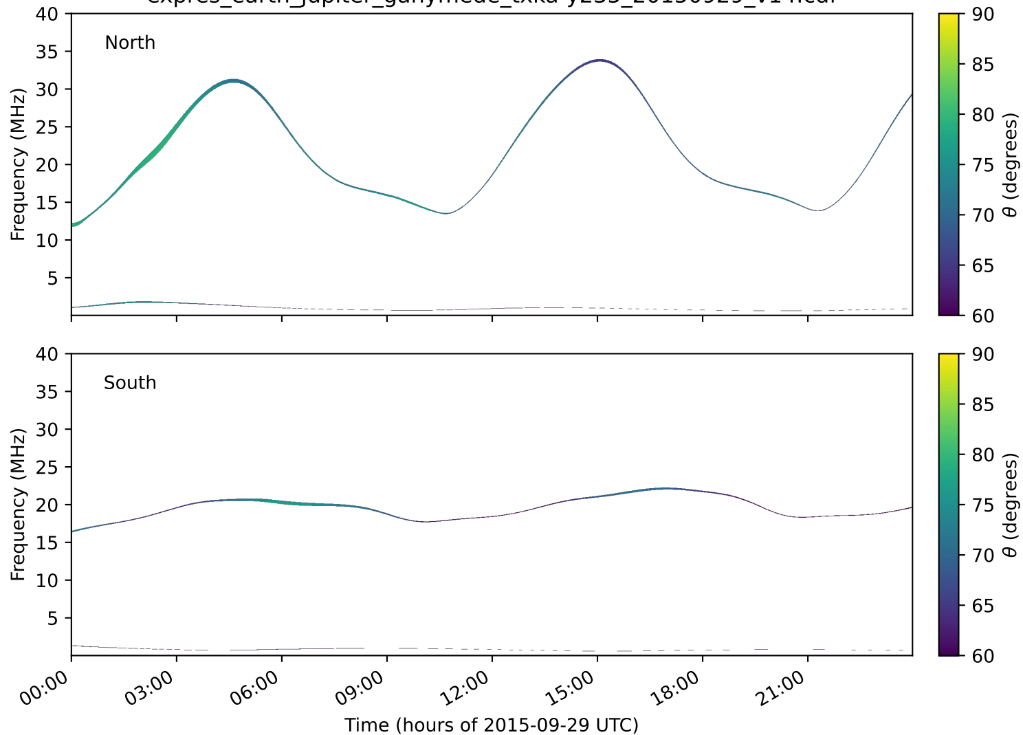
expres_earth_jupiter_ganymede_txka-y235_20150929_v14.cdf
