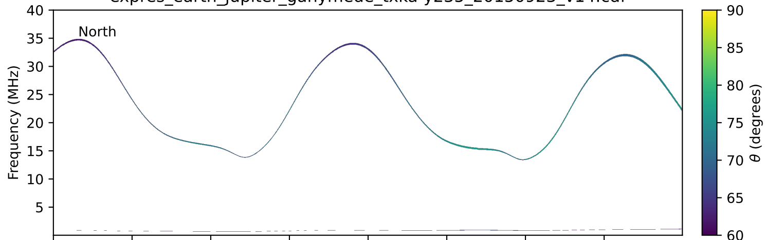
expres_earth_jupiter_ganymede_txka-y235_20150923_v14.cdf
