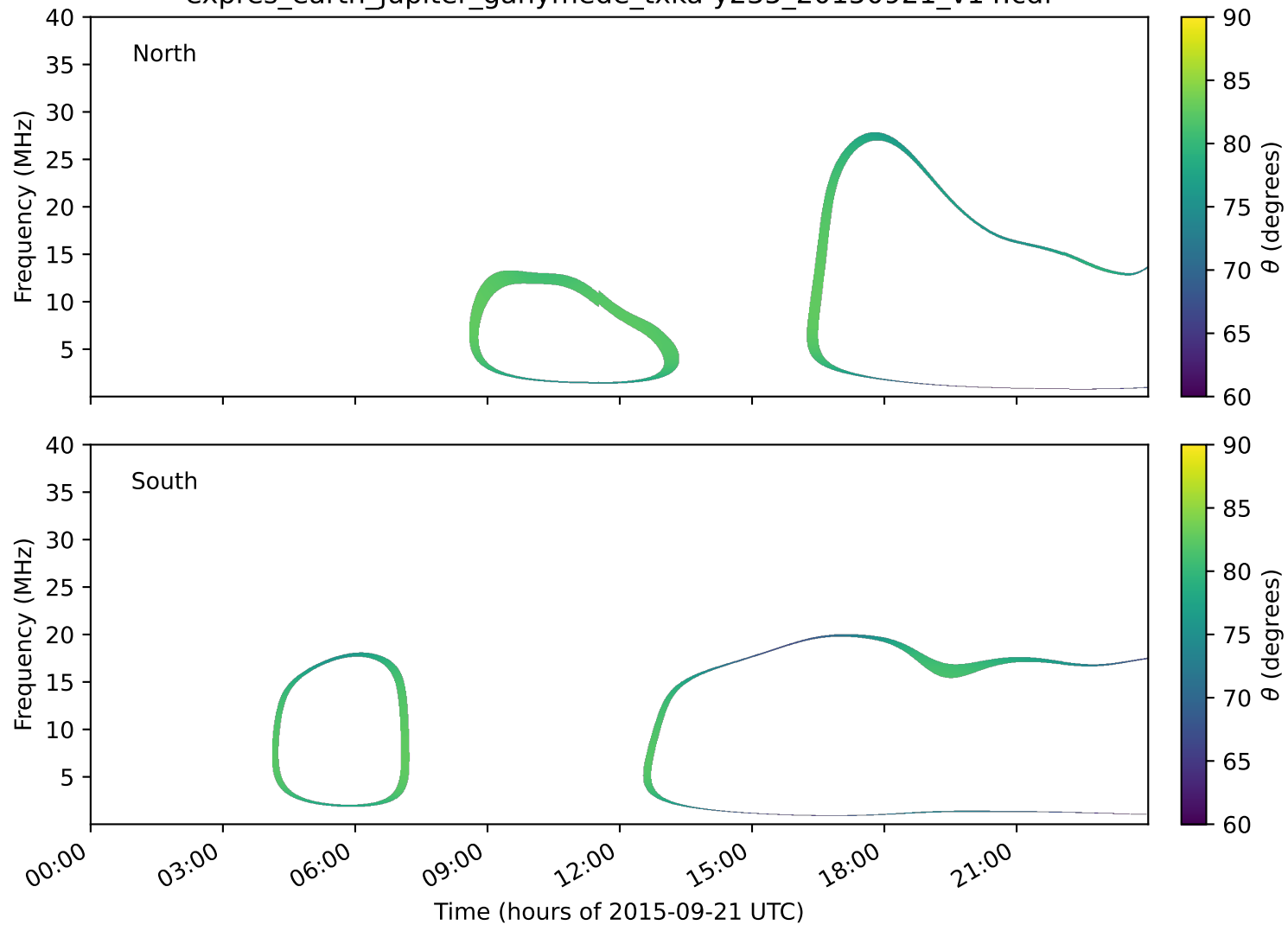
expres_earth_jupiter_ganymede_txka-y235_20150921_v14.cdf
